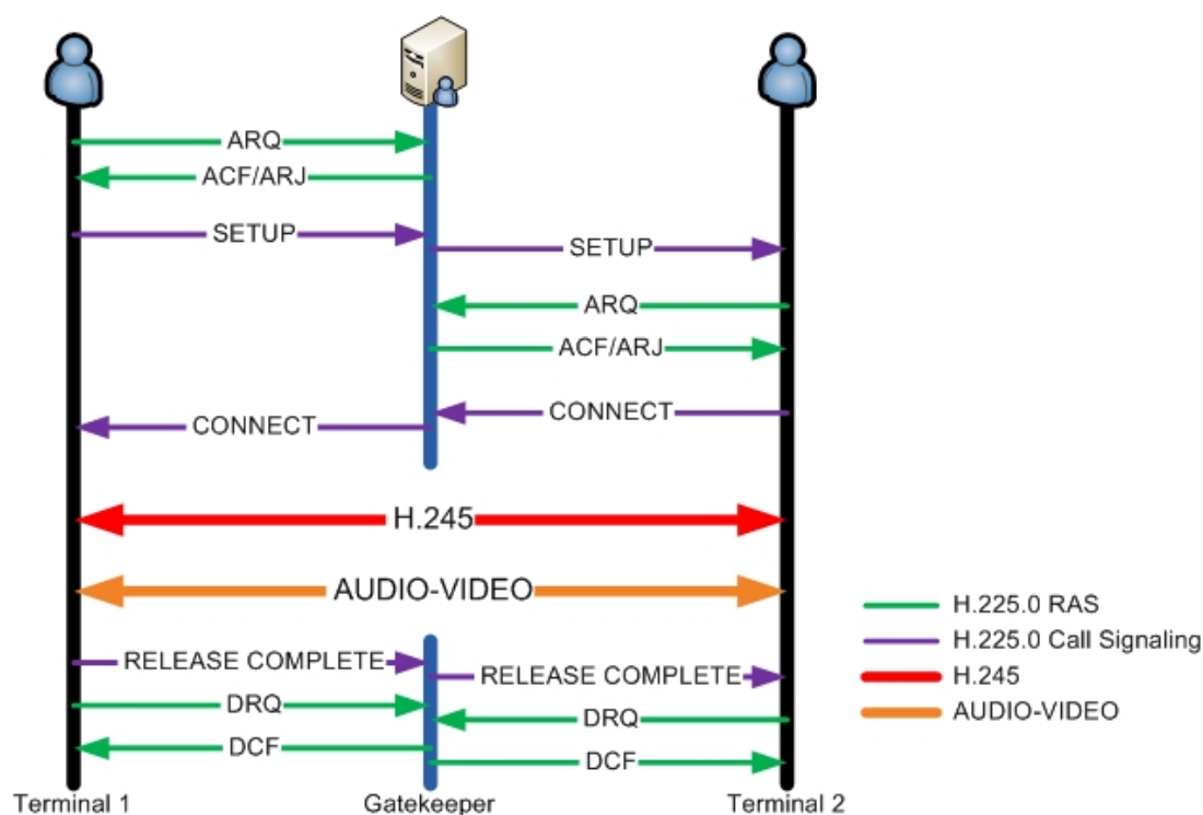
Figure 2.2: Routing the call signalling through the gatekeeper
