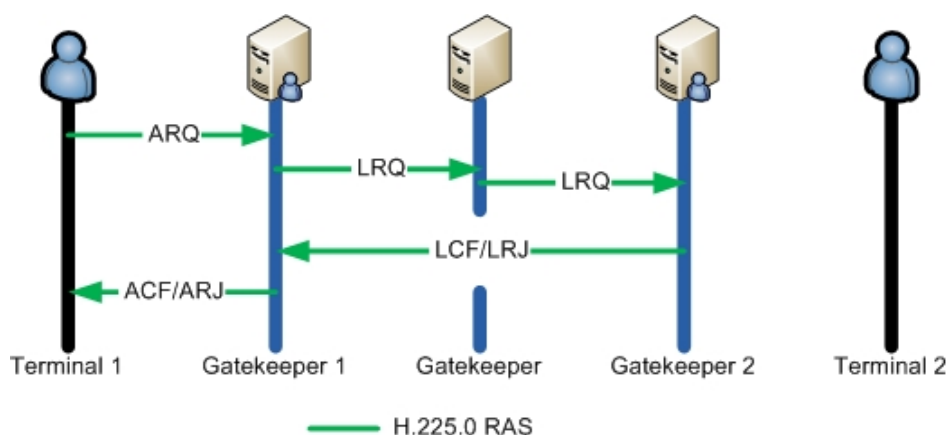
Figure 2.3: Calling a terminal from another zone
